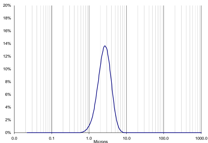
C4200 Particle Size Distribution
