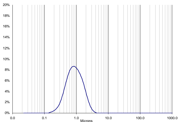
C4100 Particle Size Distribution
