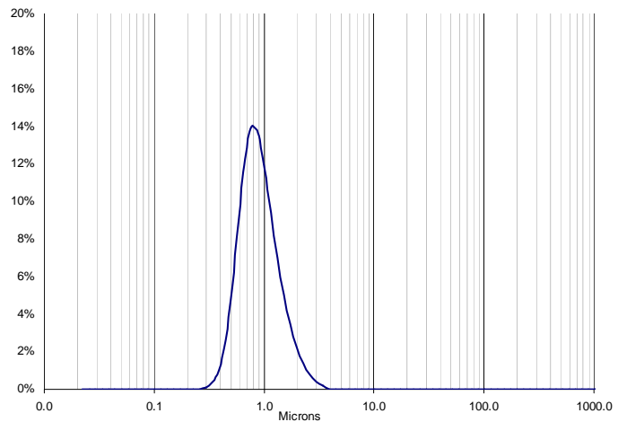
C1080 Particle Size Distribution
