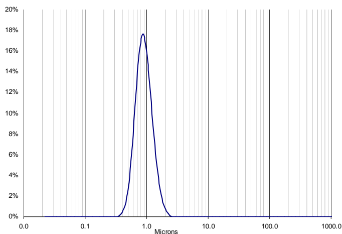
C1070 Particle Size Distribution
